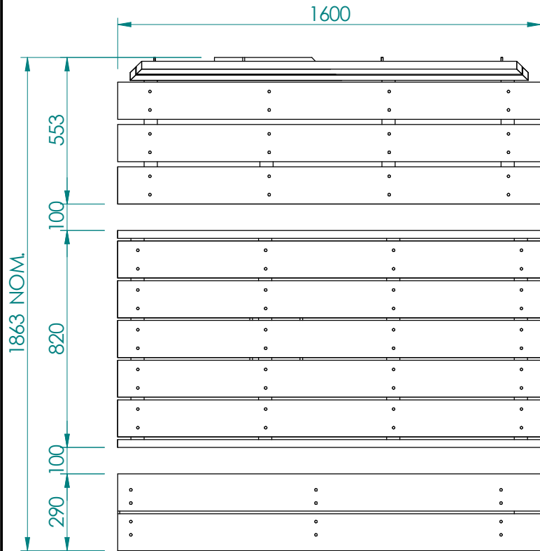
TOP VIEW
